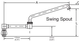
GROUP NO. 4 Double Joint
